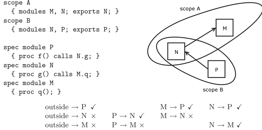
Fig. 13. Example of permissible inter-scope method calls
